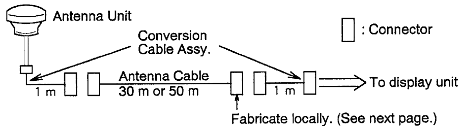
Figure 3 Installation of optional cable
